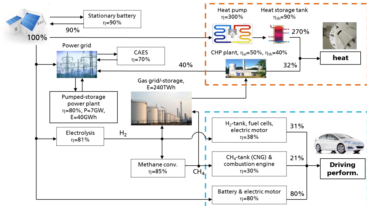
Figure 60: Possible ways of converting and storing PV power with indicative data on efficiency values.
