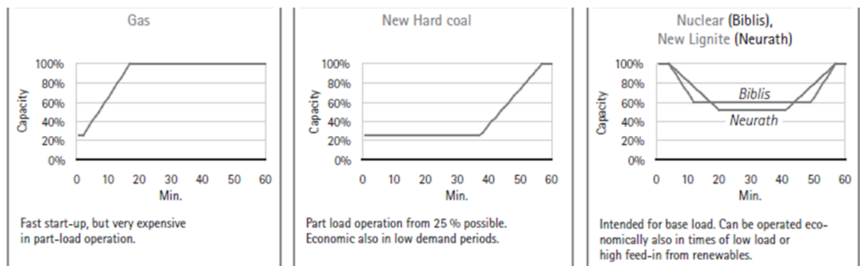
Figure 55: Power plant availability [VGB].
