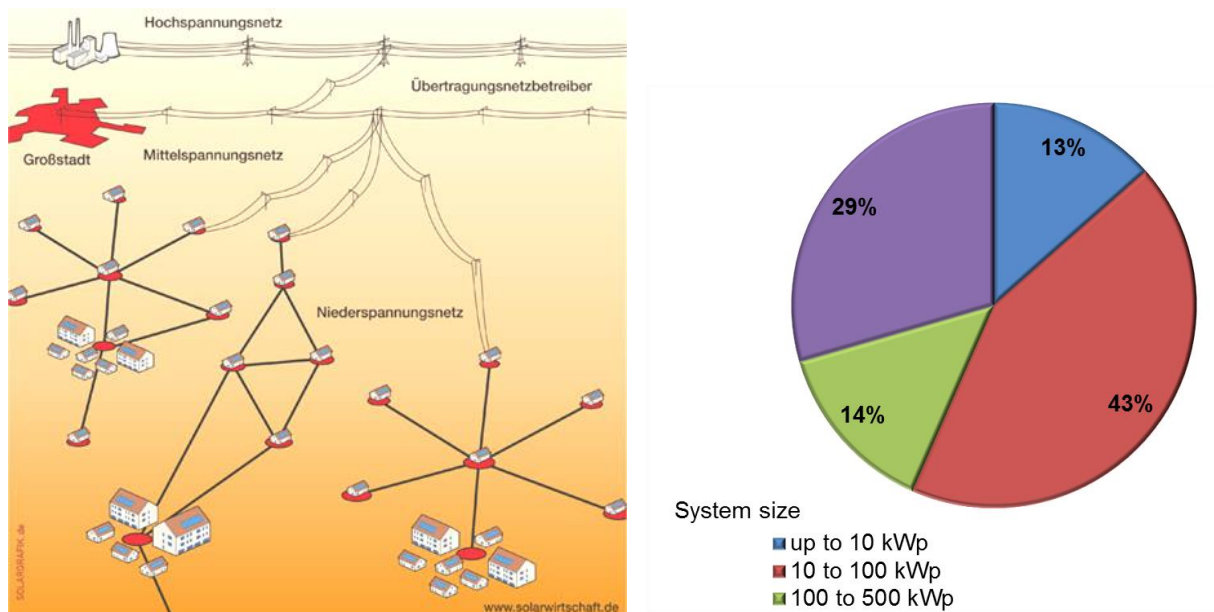
Figure 27: Left: Schema of PV power feed-in [BSW], Right: Installed PV power categorized by system size (as of Dec. 2012) (Data up to 2008 from transmission system operators (TSO), 2009: Bundesnetzagentur (German Federal Network Agency); Data compiled by PSE/Fraunhofer ISE 2013.
