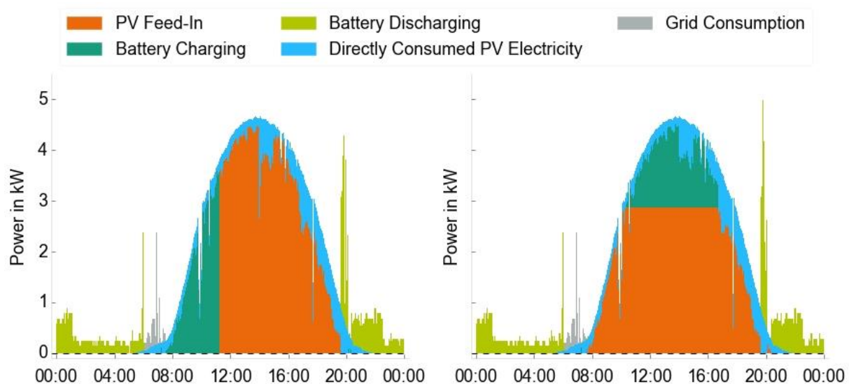
Figure 59: Comparison of the conventional and grid-optimized system operation [ISE7]
