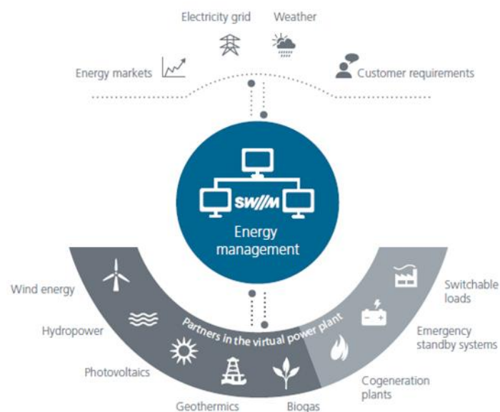
Figure 24: Concept for a virtual power plant of the Stadtwerke München (Munich municipal works) [SWM]
