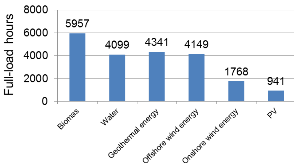
Figure 34 : Forecasted hours of full-load operation for renewable energy plants, mean values from 2012-2016
